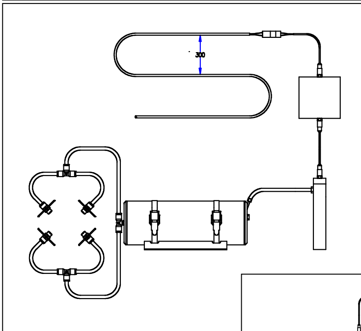
Automatic engine compartment system with Protectowire thermal sensing
